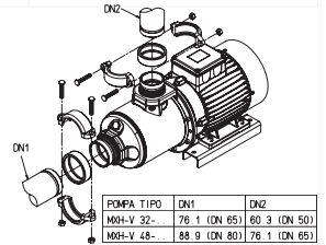
Fig. 8 Bocche con giunti Victaulic Victaulic ports Victaulic-Anschlüsse Raccordi Victaulic Acoplamiento Victaulic 进出口卡箍
